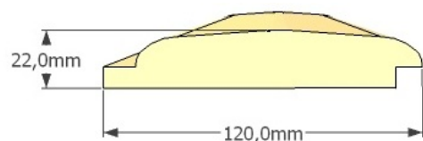
STOCKPANEL
